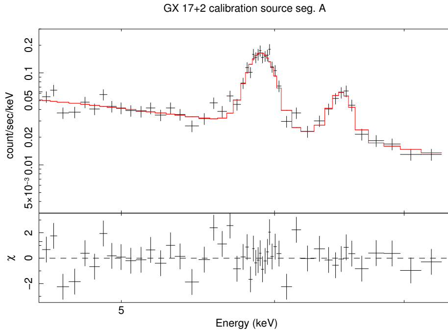
Figure 7.13: ^{55}\text{Fe} spectrum of an observation of GX17+2 performed with the 2.0s Burst option. The spectrum is fitted with a continuum plus two Gaussian lines using the response generated for the Normal mode with no Burst option.
