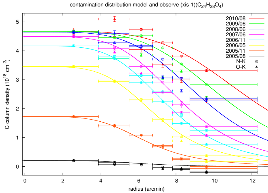
Figure 7.18: Spatial dependence of the contamination thickness derived from day Earth observations at different epochs. Open circles and filled triangles represent the data points determined by N and O lines, respectively. The best fit models are shown as solid curves.
