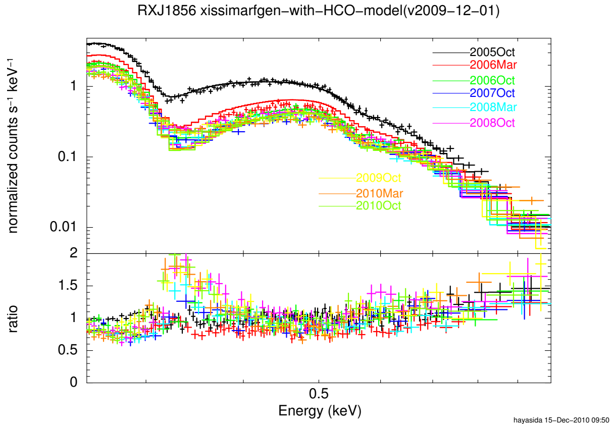
Figure 7.16: Results of spectral modeling of the BI spectrum of RX J1856.5–3754 at the XIS nominal position at several different epochs.
