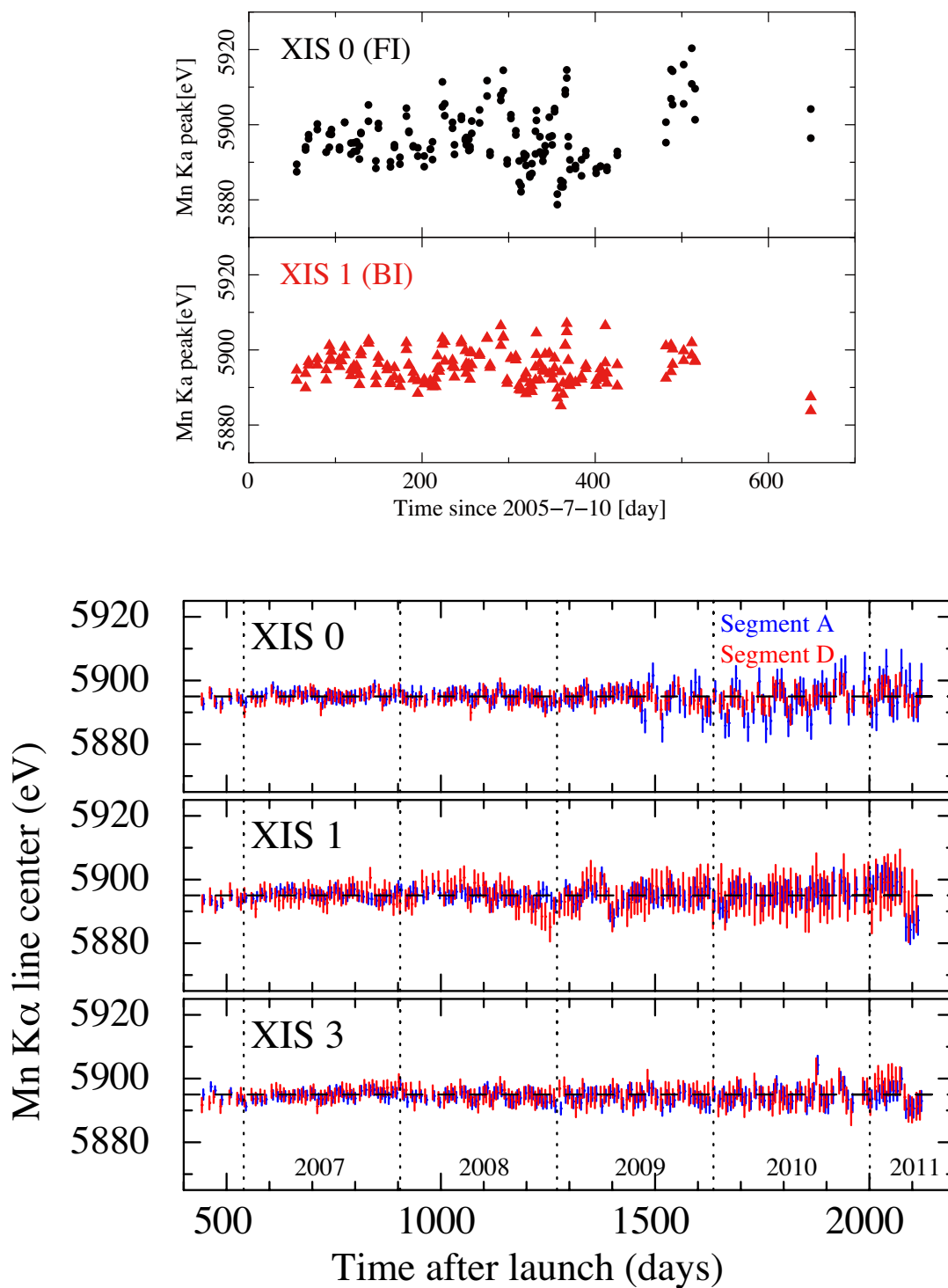
Figure 7.8: Gain in the hard band for the Normal mode (no option) using the ^{55}\text{Fe} calibration source. The upper panel shows the data before SCI-on and the lower panel after. The CTI is corrected.
