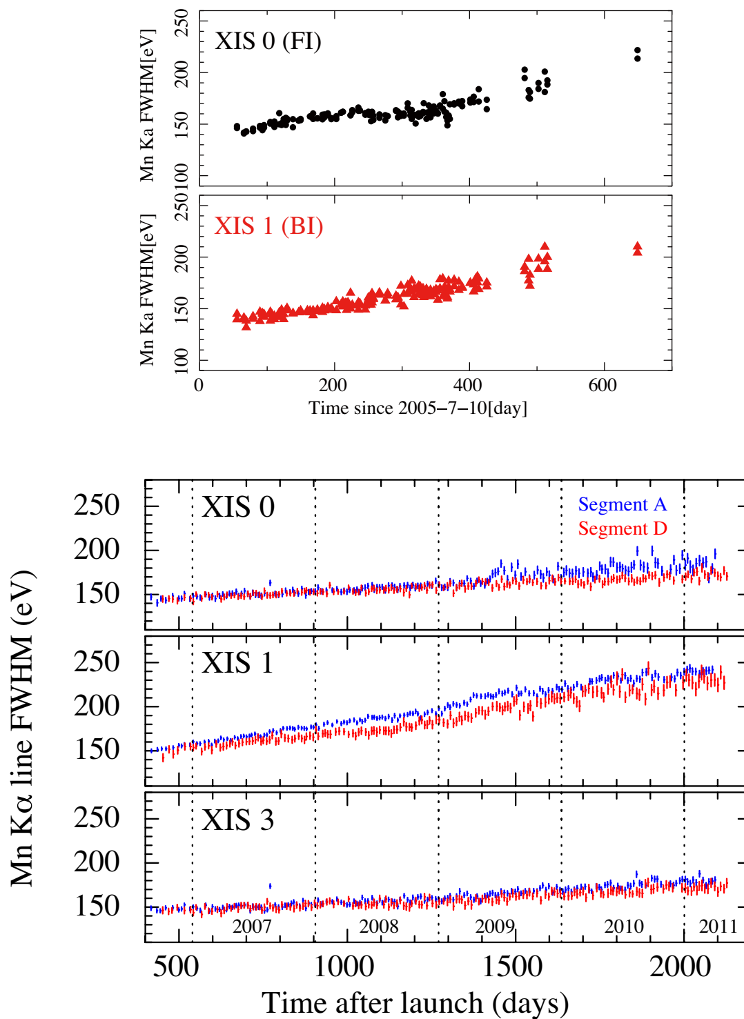
Figure 7.9: Energy resolution in the hard band for the Normal mode (without option) using the ^{55}\text{Fe} calibration source. The upper panel shows the data before SCI-on and the lower panel after. The CTI is corrected.
