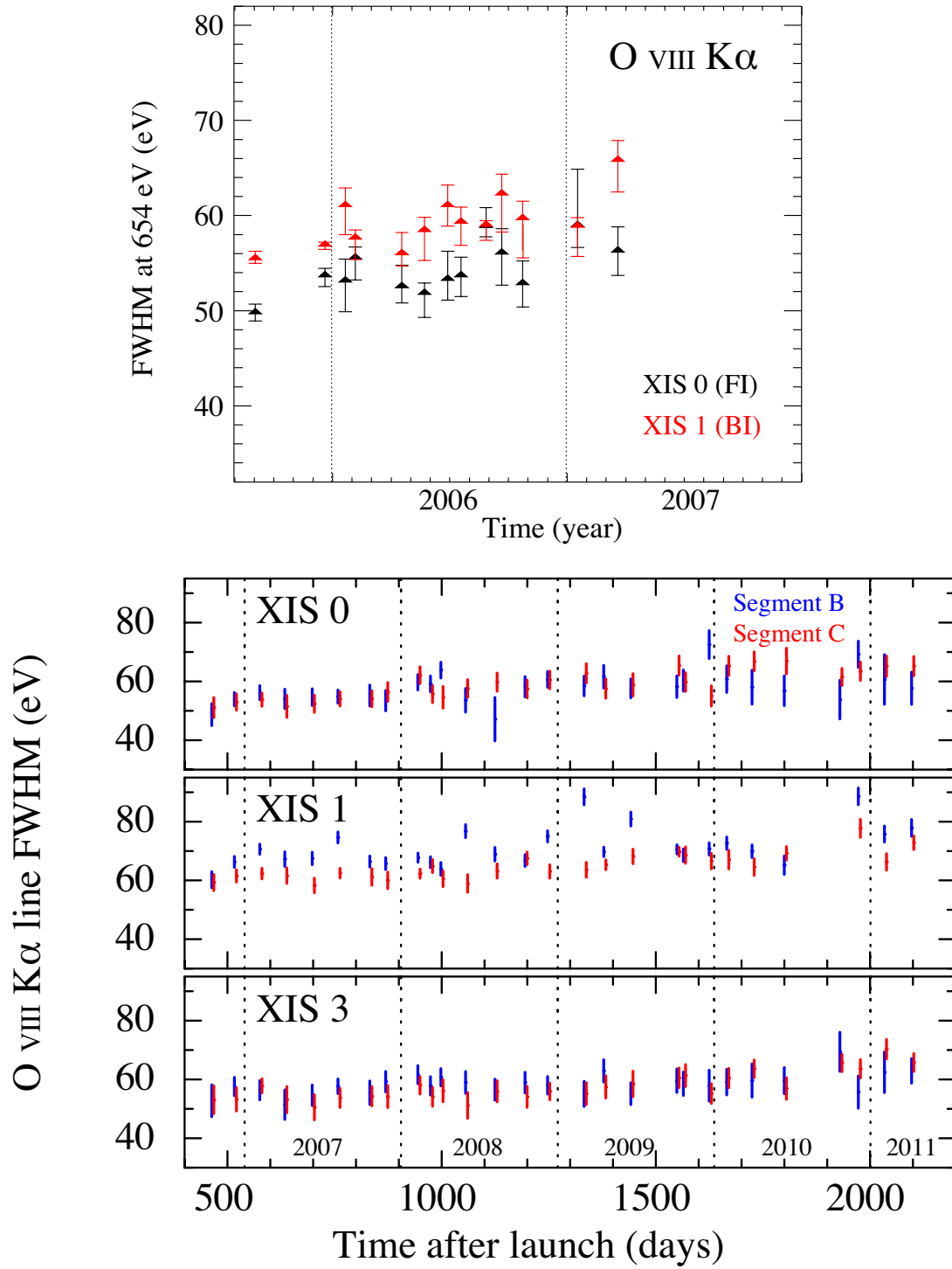
Figure 7.11: Energy resolution in the soft band for the Normal mode (without option) using E0102–72 observations. The upper panel shows the data before SCI-on and the lower panel after. The CTI is corrected.
