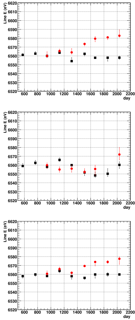
Figure 7.12: Comparison of gain in the Normal mode with the 1/4 Window option (red) and with no option (black) for XIS0 (top), XIS1 (middle), and XIS3 (bottom) using the Fe XXV K\alpha line of the Perseus Cluster.
