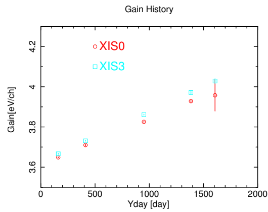
Figure 7.14: History of P-sum gain.
