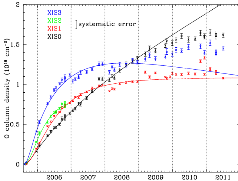
Figure 7.17: Time dependence of the contamination thickness at the XIS nominal position derived from the E0102–72 observations. The data points indicate the best fit O column density with a 90% statistical uncertainty. The curves indicate the best fit phenomenological models, based on which the calibration data base is constructed.
