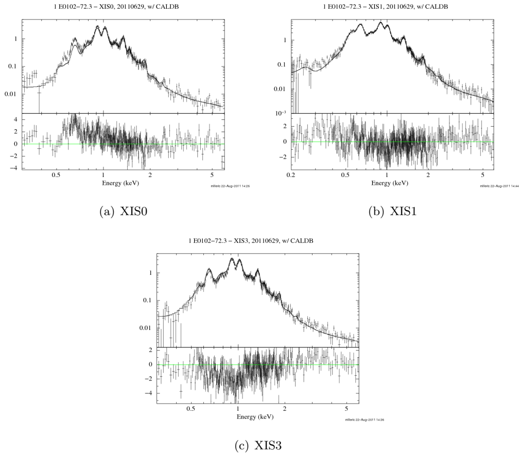
Figure 7.19: Latest results of fitting the contamination model using E0102-72 data taken on 2011-06-29.
