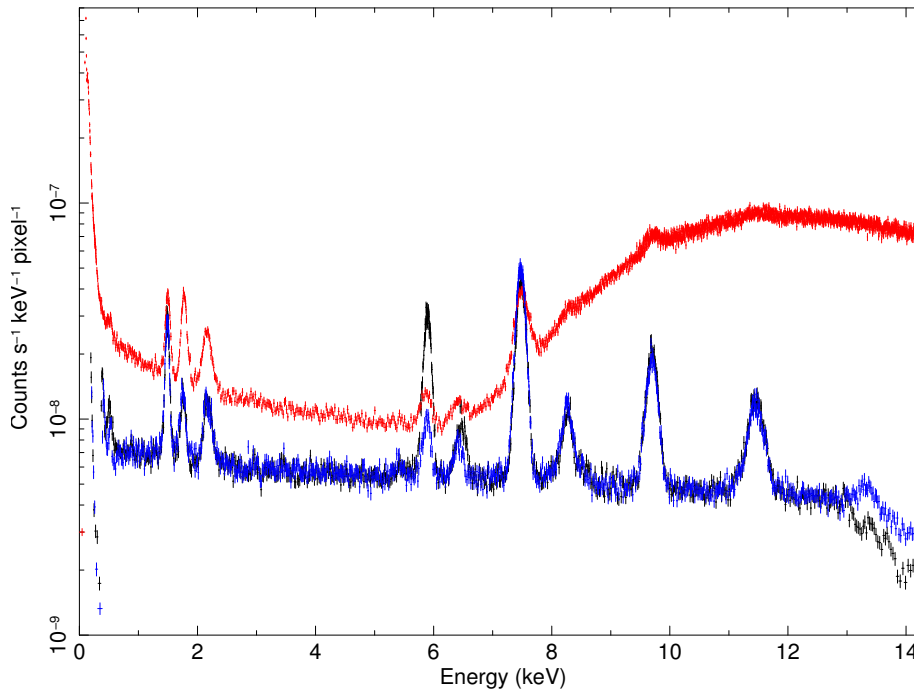
Figure 7.20: Non-X-ray background (NXB) rate for XIS0 (black), XIS1 (red), and XIS3 (blue). The spectra are constructed from night Earth observations from the SCI start to May 2010.
