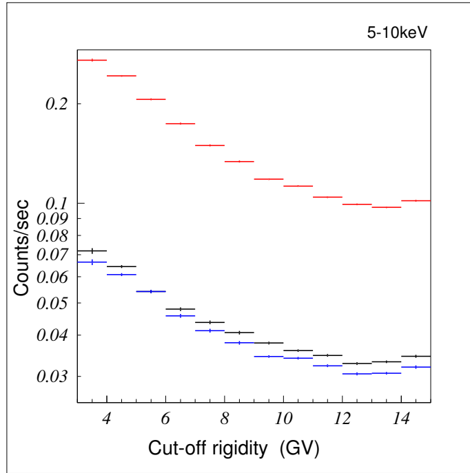
Figure 7.22: Cut-off rigidity dependence of the NXB (average intensity for 5–10 keV) for each sensor. The NXB flux varies by a factor of \sim 2 depending on the cut-off rigidity.
