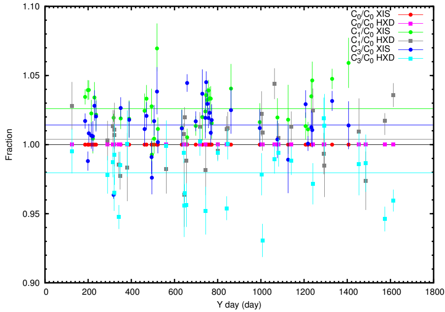
Figure 7.24: Relative flux normalization among different sensors. The ratios of the best fit normalization values for two sensors are compared at the XIS and the HXD nominal positions. Observations of a power law source in the Normal clocking mode were used. The best fit constant values are shown with solid lines.
