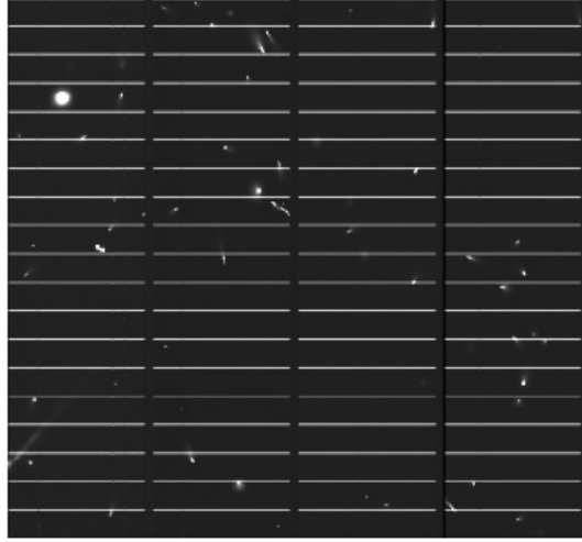
Figure 7.6: Frame dump image of XIS2 with SCI. The bright lines every 54 rows indicate rows with injected charges. Other events are mostly due to cosmic rays. The gaps between segments are due to over-clock sampling.
