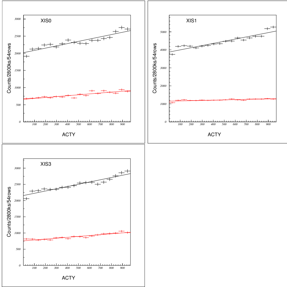
Figure 7.21: ACTY dependence of the NXB for XIS0, XIS1, and XIS3. Black lines indicate the continuum component (2.5–5.5 keV), while the red lines indicate the Ni K \alpha line component (7.2–7.8 keV). The NXB flux tends to be higher at larger ACTY, because some fraction of the NXB is produced in the frame store region.
