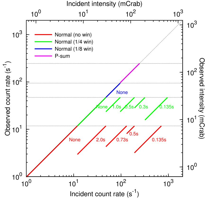
Figure 7.23: Incident vs observed count rates of a point source for the FI sensors. The thick colored lines indicate the ranges that can be observed without pile-up.
