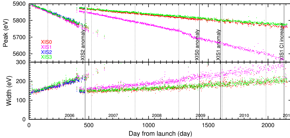
Figure 7.7: Trend of ^{55}\text{Fe} peak height and width. These are raw values without trail correction. See Fig. 7.9 for the gain and energy resolution for calibrated data.
